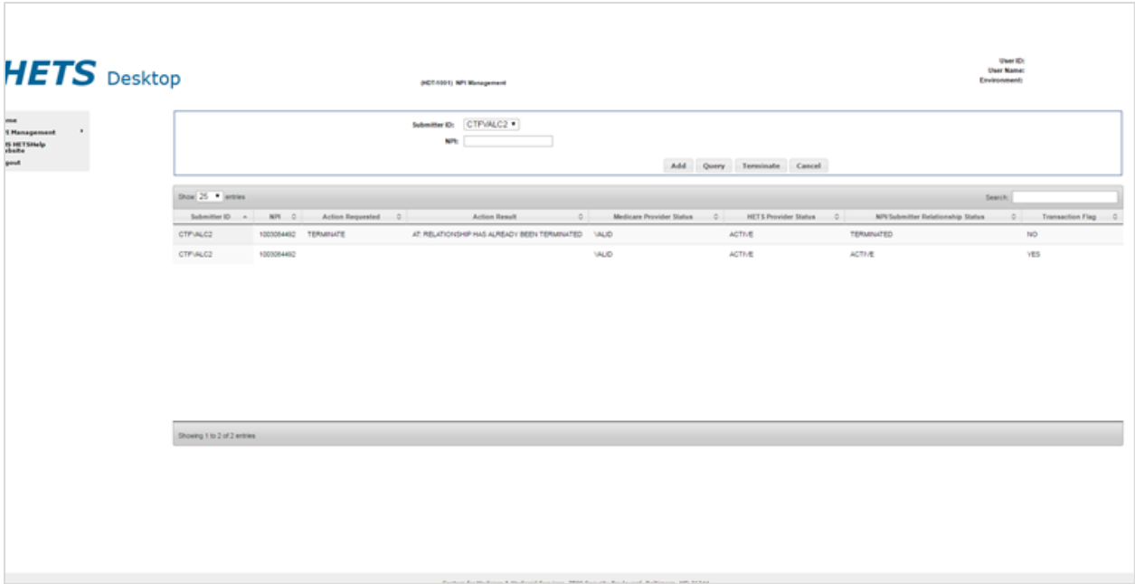
Figure 91: HDT NPI Management Screen (HDT-1001) – Terminate Results
